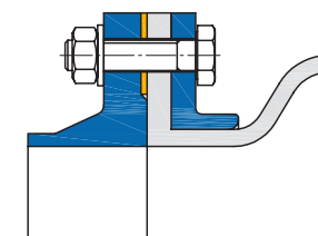
Version 3 with recess spacer ring
