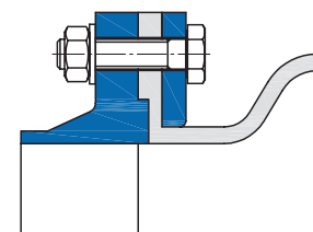
Version 2 with recess compensation
