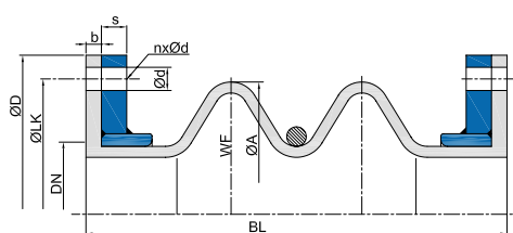
Example - double corrugation, Design A - without tie rods
